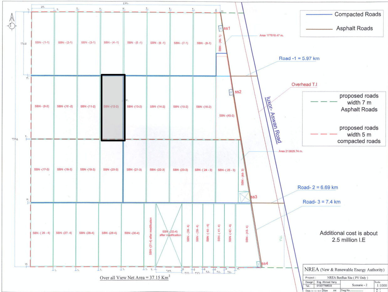
Figure 3-2: Scatec Solar - Kom Ombo Renewable Energy Project (plot 12-2)
